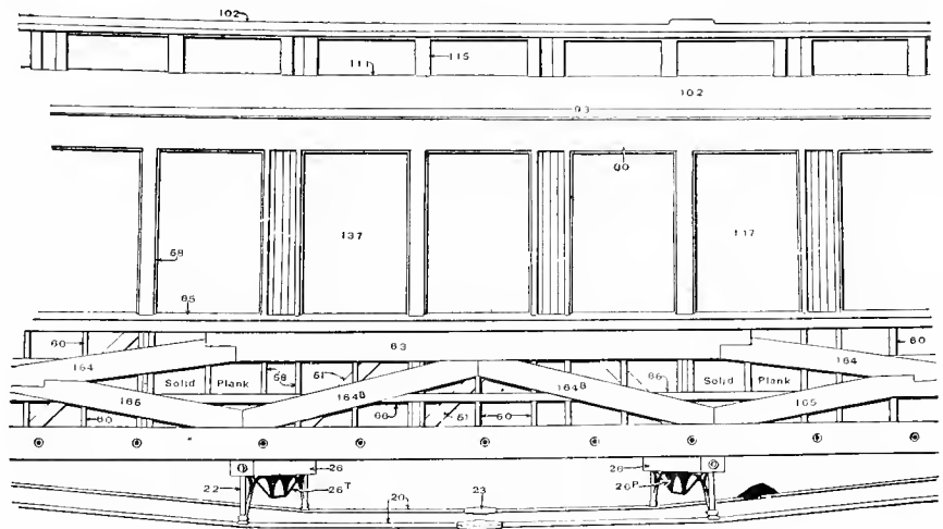
Fig. 536. Part Side Elevation.
